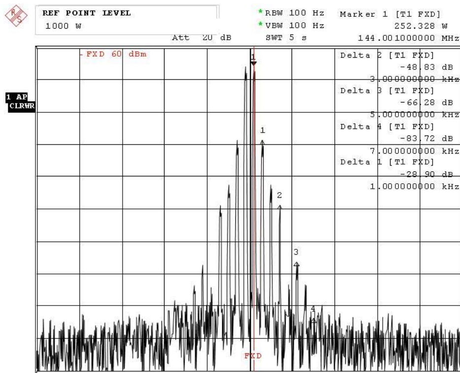
Figure 6. 1000 W PEP Two-Tone Spectrum
